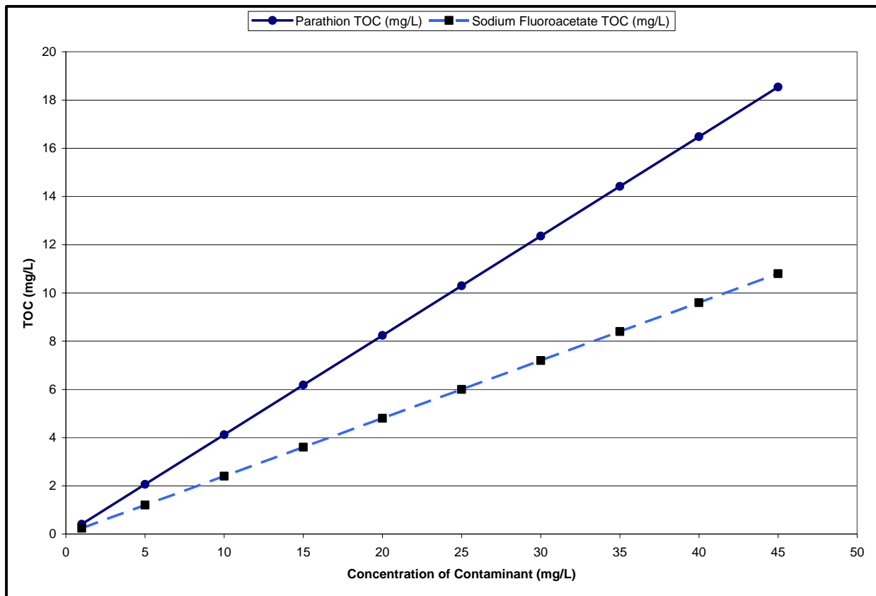
Figure 2: TOC Changes with Addition of Organic Contaminants to Tap Water
