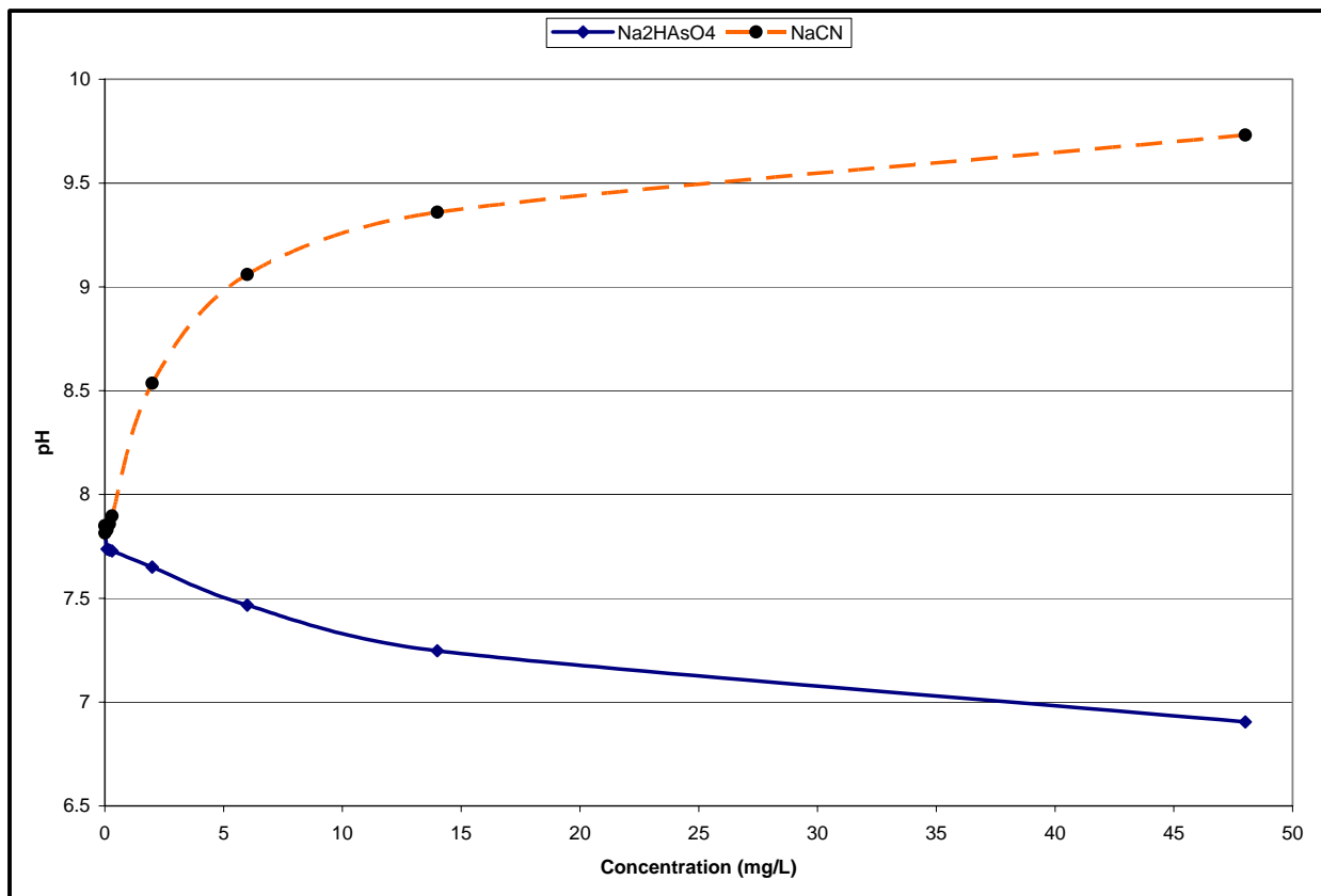
Figure 1: pH Changes with Addition of Inorganic Contaminants to Tap Water
